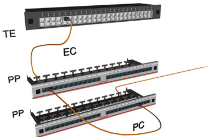
Fig. 5. Example of cross-connect type
