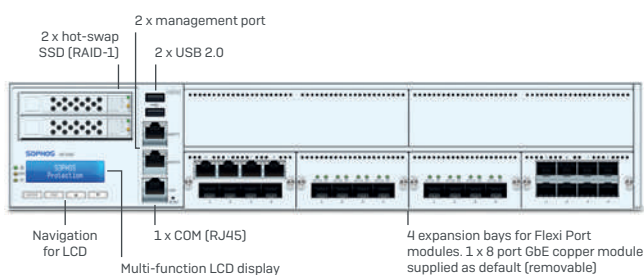
Front View XG 650
